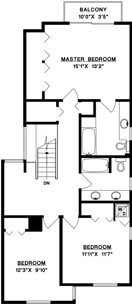
UPPER FLOOR
